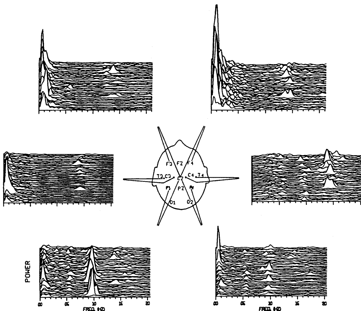
Figure 6. Compressed spectral arrays showing 10 minutes of spectral analyzed EEG data from bipolar montage referenced to Cz during right central SMR training session in a nonepileptic subject. Successive 8 sec. epochs are shown. Note spectral density peaks at 13-15 Hz from central and frontal recordings, greatest on the right. Parietal 9-11 Hz activity is seen also, greatest on the left. Peaks at 0.5-2 Hz reflect eye-blink artifact. (Modified from reference 19)
